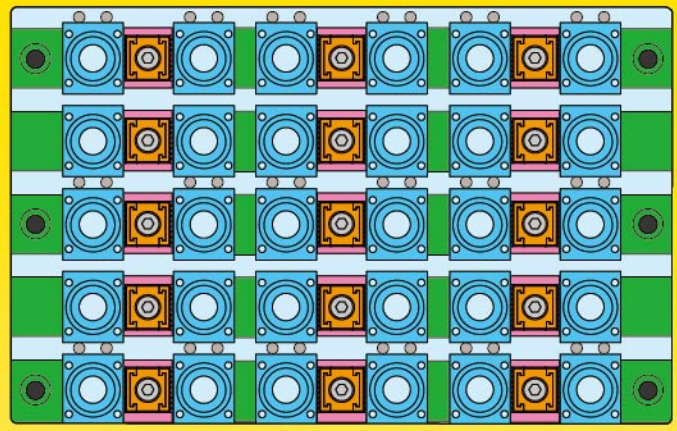
► Little King Kong Vise: An example of fixing square work-piece.
